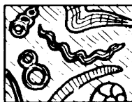
Biosparite and Biosparrudite (Ib)
