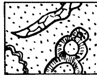
Biomicroite and Biomicrodite (IIb)
