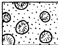
Oomicrite and Oomicrudite (IIo)
