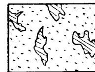
Dismicroite (III x )
