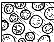
Oosparite and Oosparrudite (Io)
