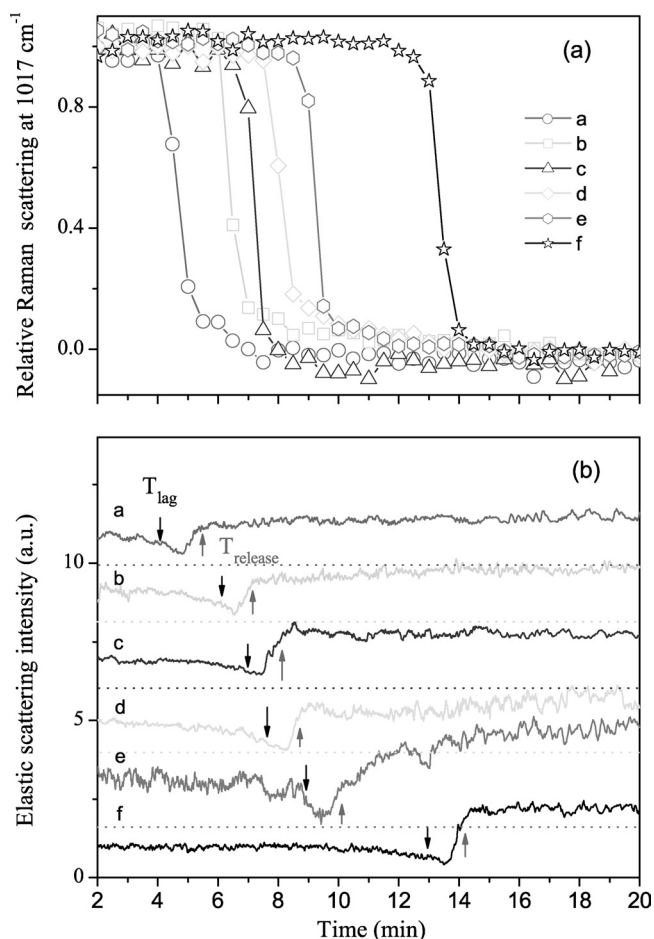
FIG. 5. CaDPA release and ELS intensities for six individual B. cereus spores during wet-heat treatment at 80°C. (a) Relative intensities of the CaDPA-specific Raman band at 1,017 \text{cm}^{-1} for six individual spores (spores a to f) were determined as described in Materials and Methods. (b) Relative ELS intensities of the six spores described in the legend for panel a were determined as described in Materials and Methods. The baselines of ELS intensity were shifted for display, and the dashed line below each ELS signal is the corresponding zero level. The downward and upward arrows mark T_{\text{lag}} and T_{\text{release}} , respectively, for each spore.
