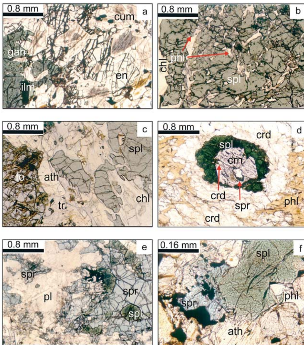
FIG. 5. Plane-polarized transmitted-light photomicrographs of textural relationships involving zincian spinel from Colorado. a. Gahnite (gah) – cummingtonite (cum) – enstatite (en) – zincian ilmenite (ilm) rock (Green Mountain). b. Phlogopite (phl) and chlorite (chl) on the margins of and as inclusions in zincian spinel (spl) (Cotopaxi). c. Zincian spinel – anthophyllite (ath) – forsterite (fo) – tremolite (tr) assemblage in contact with retrograde chlorite (Caprock). d. Corundum (crn) with sapphirine (spr) and cordierite (crd) inclusions mantled by spinel and surrounded by cordierite and phlogopite (Marion). e. Spinel – sapphirine – plagioclase (pl) assemblage (Amethyst). Note the spinel inclusion in sapphirine. f. Sapphirine surrounding spinel next to anthophyllite and phlogopite (Unnamed prospect).
