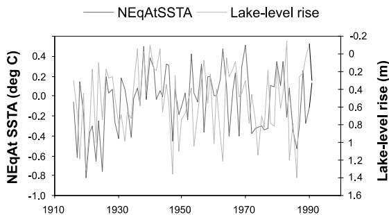
Fig. 5. Time series of annual rise of level of Lake Titicaca compared with the time series of DJFM Sea Surface Temperature (SST) anomaly for the northern equatorial Atlantic (7.5° to 22.5°N, 2.5°E to 37.5°W; SST anomaly data from Kaplan et al., 1997). Colder SSTs in the northern equatorial Atlantic correlate with wet conditions in much of Amazonia (Nobre and Shukla, 1996) and in the northern Altiplano.
