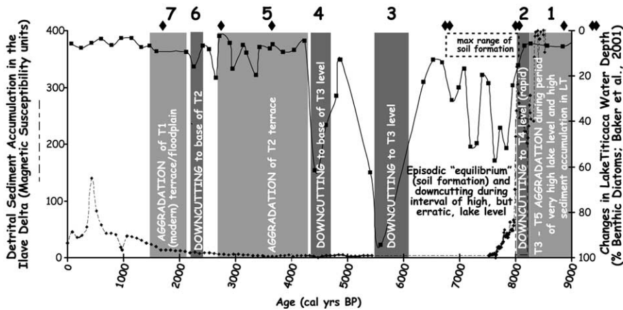
Fig. 12. Relationship between the Rio Ilave terrace development and changes in base level and sediment load. The benthic diatom record from a deep-water core (NE98-2PC) in Lake Titicaca is used as a proxy for lake level (solid line). The magnetic susceptibility log from a core taken at the toe of the Ilave delta records detrital sediment accumulation at base level (dashed line). The diamonds indicate radiocarbon dates in the fluvial sequence and the numbers correspond to the aggradational and downcutting events illustrated in Fig. 11. Note that periods of aggradation correspond to periods of high (or rising) lake level in Lake Titicaca (Abbott et al., 1997; Baker et al., 2001a) and (for all but T2) the periods of increased sediment accumulation in the Ilave delta. Further, each hypothesized aggradation period corresponds to a lacustrine period in the Rio Desaguadero valley (Baucom and Rigsby, 1999; Rollins, 2001). Downcutting episodes, which leave behind no datable strata, are bracketed in age by dates within the aggradational sequences and apparently correspond to periods of low lake level in Lake Titicaca (Baker et al., 2001a), low or rapidly decreasing sedimentation rates in the Ilave delta, and fluvial activity in the Rio Desaguadero valley (Baucom and Rigsby, 1999; Rollins, 2001).
