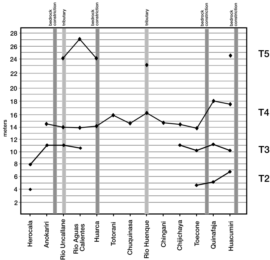
Fig. 10. Graph showing the heights of the four upper Rio Ilave terrace tracts. Terrace height is partially controlled by proximity to bedrock constrictions and tributaries.
