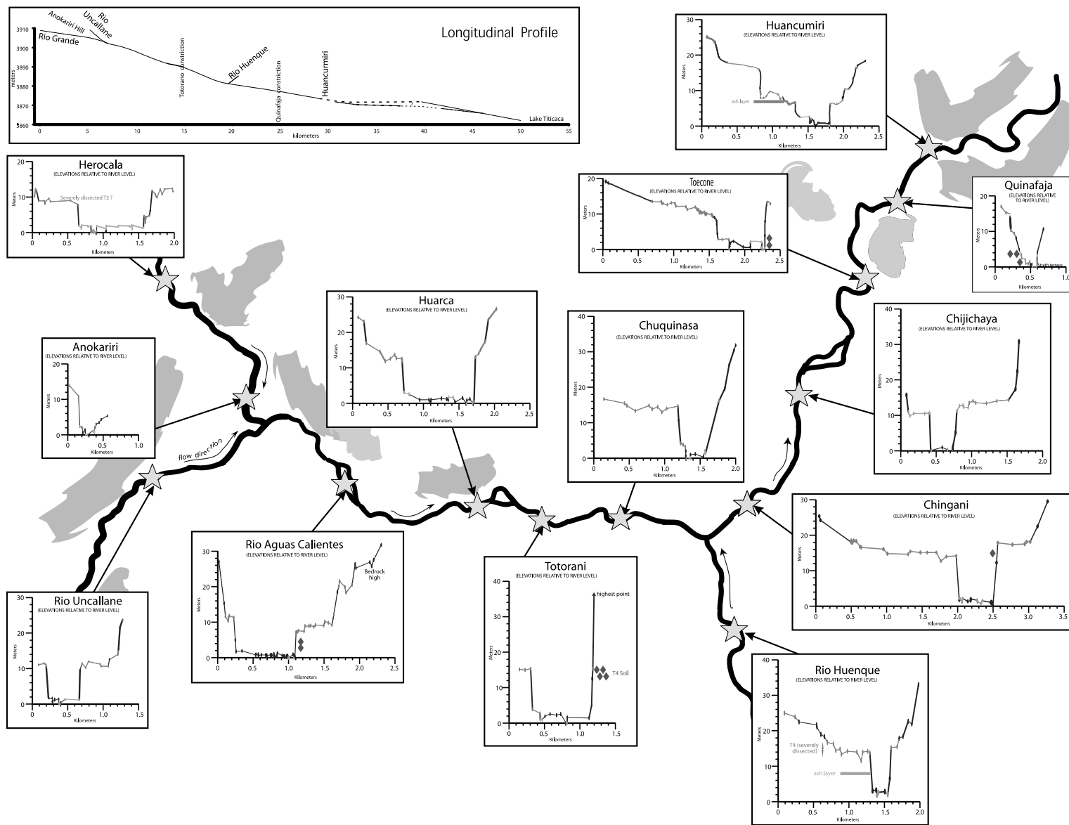
Fig. 7. Rio Ilave terrace profiles and longitudinal profile. Diamonds mark locations of key dates; shaded areas show bedrock highs.
