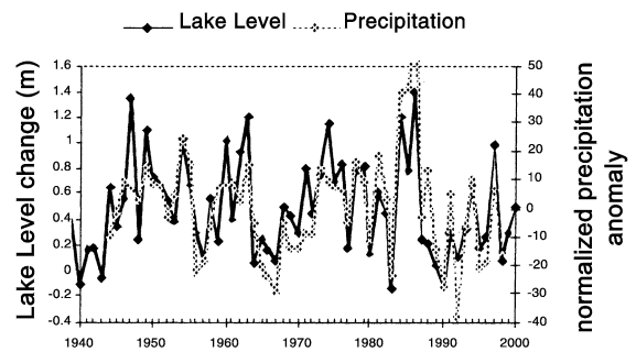
Fig. 3. Annual rise of lake level (October–April) is correlated with the instrumental record of annual precipitation within the northern Altiplano (normalized rainfall departures from 20 stations in the Lake Titicaca watershed): lake level rise is a good measure of precipitation integrated throughout the basin. ENSO and quasi-decadal fluctuations of lake level are evident.
