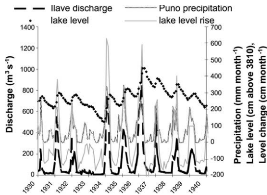
Fig. 2. The level of Lake Titicaca has been recorded at Puno, Peru, since 1914. The highly seasonal nature of the rainfall on the Altiplano causes increased input to the lake (as illustrated by the Ilave discharge) and a sharp lake level rise near the end of the wet season. This rise is followed by a slower, evaporation-driven, fall of lake level spread over the remainder of the year and, at high lake stages, discharge via the Rio Desaguadero.
