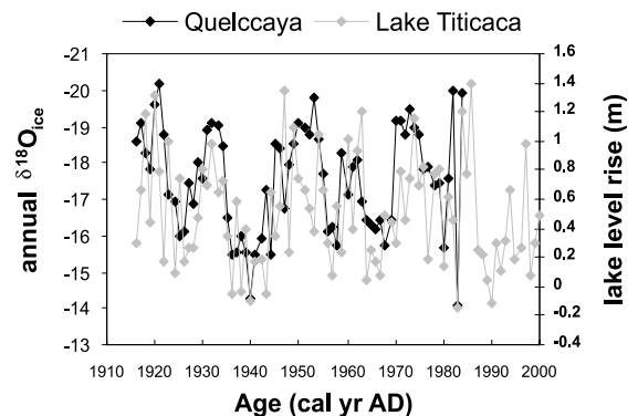
Fig. 4. There is a significant correlation between the \delta^{18}\text{O}_{\text{ice}} from Quelccaya and annual lake level rise ( r^2=0.2424 , n=69 , significant at the 99% confidence level), a less significant correlation between layer thickness at Quelccaya and lake level rise ( r^2=0.1558 , n=69 ), and no significant correlation between \delta^{18}\text{O}_{\text{ice}} and layer thickness for the period 1500–1984 ( r^2=0.0125 , n=485 ). Thus, \delta^{18}\text{O}_{\text{ice}} is an excellent proxy for past precipitation; ice layer thickness is not.
