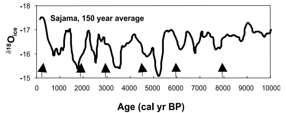
Fig. 6. \delta^{18}\text{O}_{\text{ice}} in the Sajama ice cap (Thompson et al., 1998), three-point moving average of presumed 50-yr intervals. Millennial events of 1–1.5‰ amplitude are persistent throughout the Holocene. The arrows highlight the millennial cold SST events deduced from sediment cores offshore West Africa (DeMenocal et al., 2000) and synchronous with the ‘Bond events’ of the subpolar North Atlantic (Bond et al., 2001). Baker et al. (2001b) hypothesized that tropical Atlantic meridional SST gradients force millennial wet–dry cycles in the Lake Titicaca watershed.
